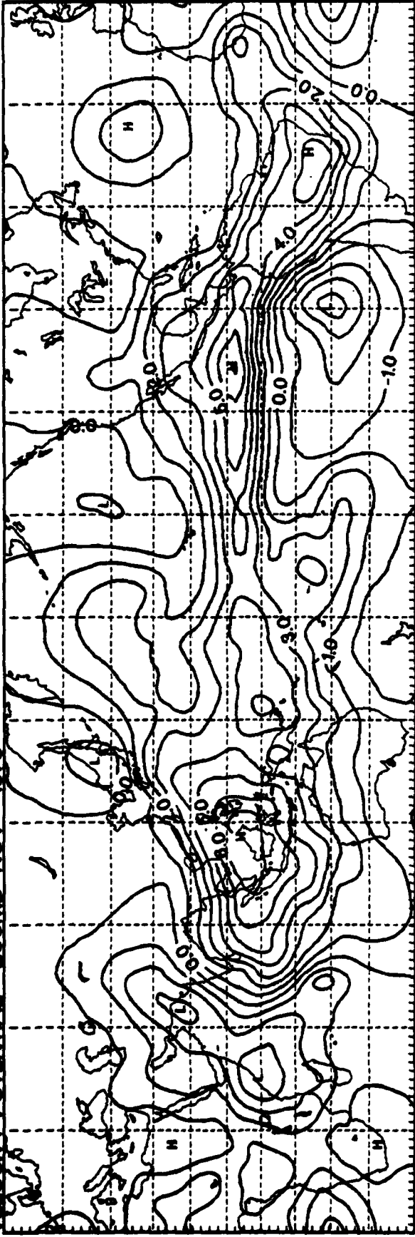
VELOCITY POTENTIAL 200MB NOV 1976
